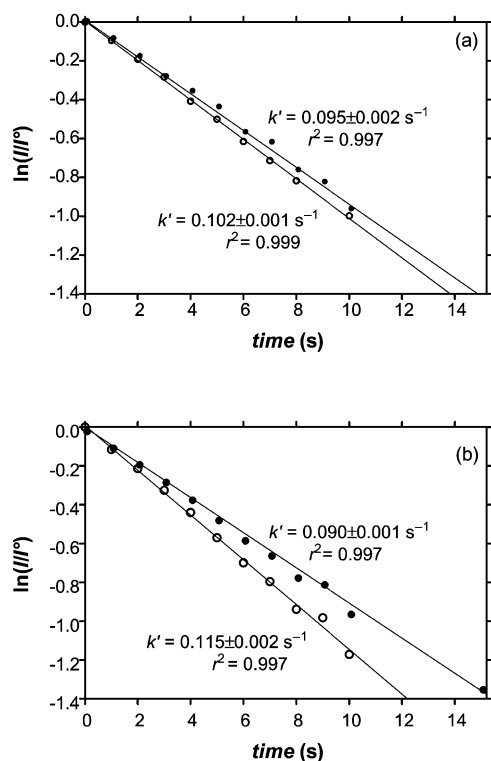
Figure 6. (a) Kinetic plots for the gas-phase reaction between (R)-(-)-2-butylamine ( P_B = 4.6 \times 10^{-8} mbar) and [4 \cdot H \cdot L-tyr^{OMe}]^+ (open circles) or [ent-4 \cdot H \cdot L-tyr^{OMe}]^+ (full circles); (b) kinetic plot for the gas-phase reaction between (S)-(+)-2-butylamine ( P_B = 4.6 \times 10^{-8} mbar) and [4 \cdot H \cdot L-tyr^{OMe}]^+ (open circles) or [ent-4 \cdot H \cdot L-tyr^{OMe}]^+ (full circles).
