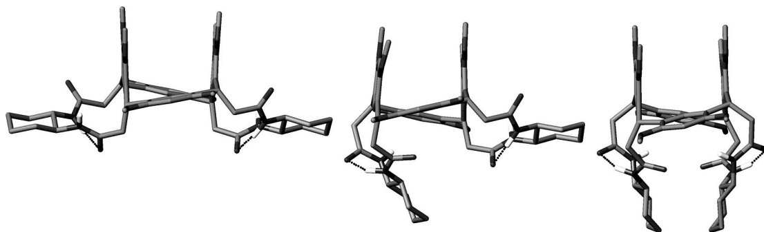
Figure 2. Lowest energy conformers of basket resorcin[4]arene 3 from MCMM and MCMM/LCMS calculations. Left to right 3a , 3b , and 3c (in order of increasing energy).
