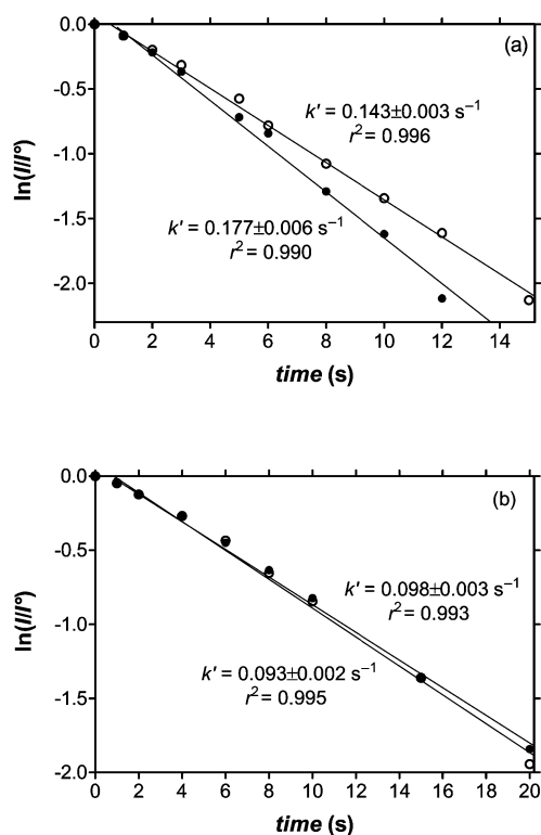
Figure 7. (a) Kinetic plots for the gas-phase reaction between (R)-(-)-2-butylamine ( P_B = 7.2 \times 10^{-8} mbar) and [ent-4 \cdot H \cdot L-amph]^+ (open circles) or [4 \cdot H \cdot L-amph]^+ (full circles); (b) kinetic plot for the gas-phase reaction between (S)-(+)-2-butylamine ( P_B = 4.7 \times 10^{-8} mbar) and [ent-4 \cdot H \cdot L-amph]^+ (open circles) or [4 \cdot H \cdot L-amph]^+ (full circles).
