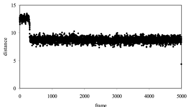
Figure 4. Distance between two dummy atoms corresponding to the center of the bond connecting the two phenyl-substituted carbon atoms of each wing estimated during the SD run for 4a .
