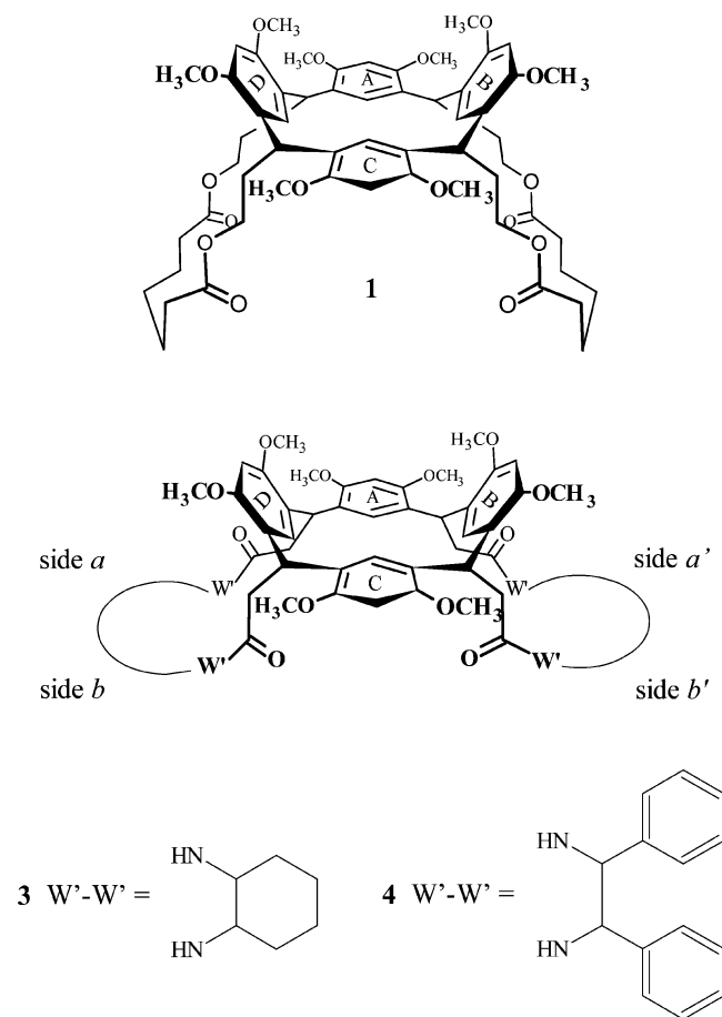
Figure 1. Chemical structures of a basket resorcin[4]arene with two polymethylene bridges ( 1 ) [10] and of chiral basket resorcin[4]arenes 3 and 4 .
