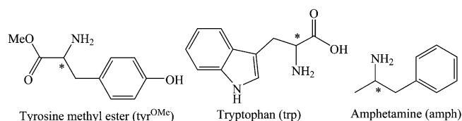
Figure 5. Chemical structures of chiral guests A.
