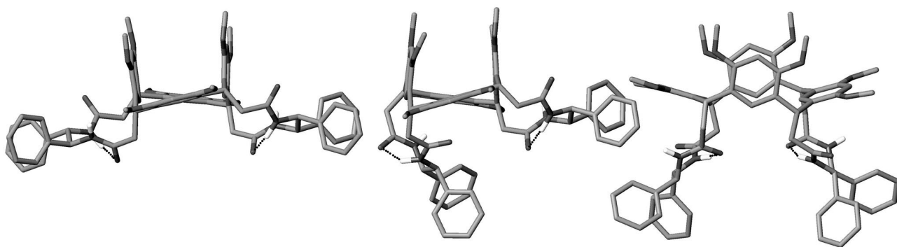
Figure 3. Lowest energy conformers of basket resorcin[4]arene 4 from MCMM and MCMM/LCMS calculations. Left to right 4a , 4b , and 4c (in order of increasing energy).
