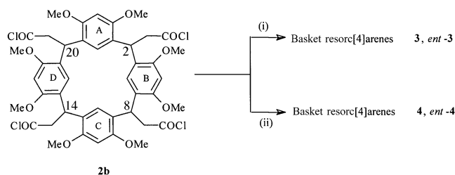
Scheme 2. Reagents and conditions: (i) DIPEA, dry THF, 1,2-DACH, reflux, 3 h; (ii) DIPEA, dry THF, 1,2-DPEDA, reflux, 3 h.
