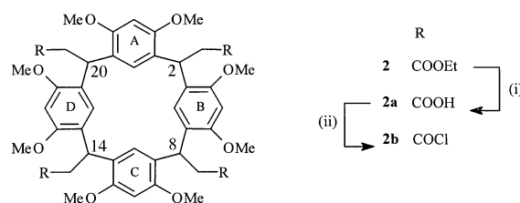
Scheme 1. Reagents and conditions: (i) 2 N NaOH, EtOH, reflux, 4 h, glacial AcOH; (ii) thionyl chloride, dry benzene, reflux, 4 h.
